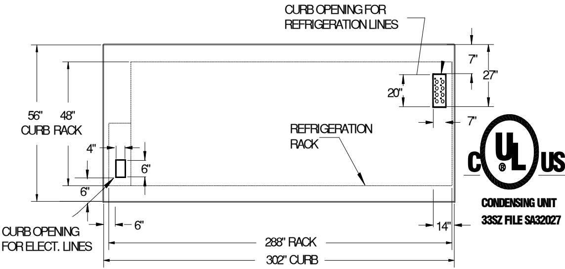
PLAN VIEW
